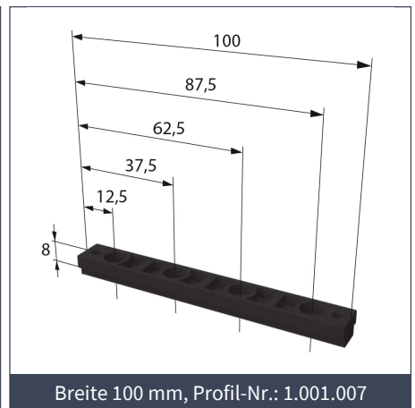
T-Profil, Material PAN1, schwarz
